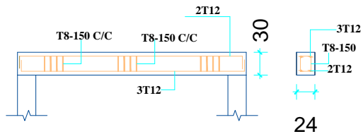
INVERTED BEAM IB : 24x30
