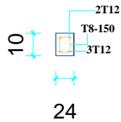
CONCEALED BEAM - CB : 24x10
